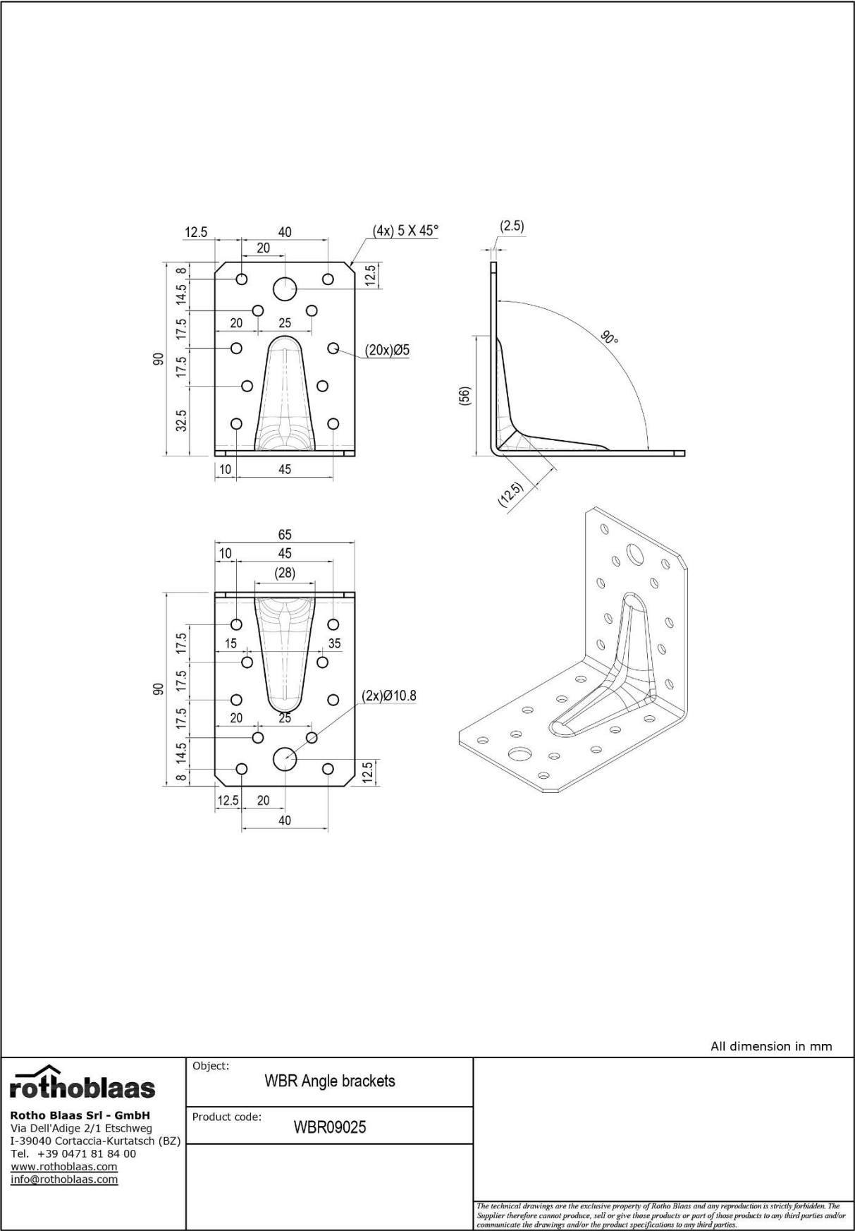
Figure B.4 Dimensions of Angle Bracket WBR09025
