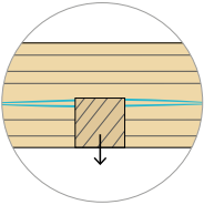
HANGING LOAD tension reinforcement perpendicular to grain
