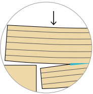
NOTCH tension reinforcement perpendicular to grain
