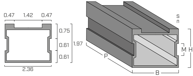
ALU TERRACE 50
