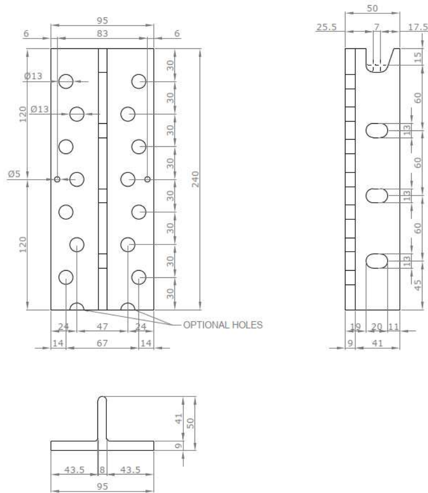
Drawing: ALUMEGA 240 HP
