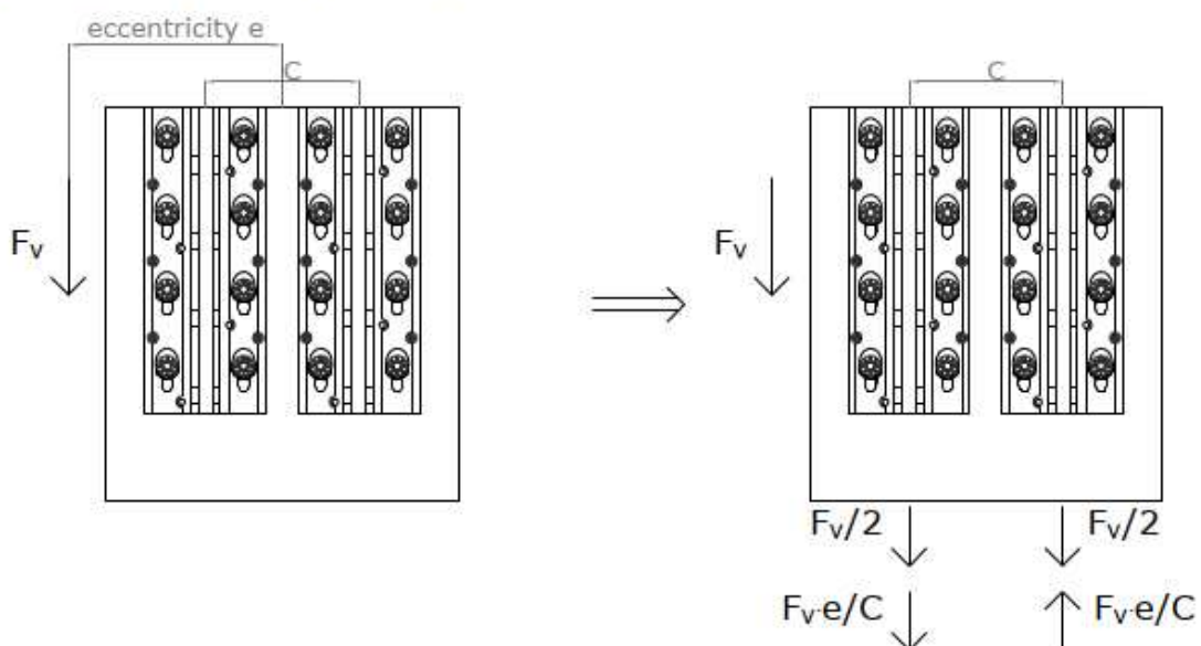
Eccentric force on the joist connectors
