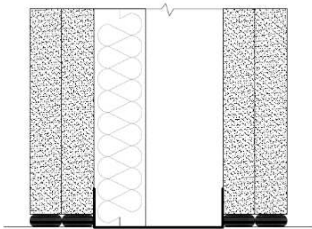
Figure 7 - Conf. 4 scheme
