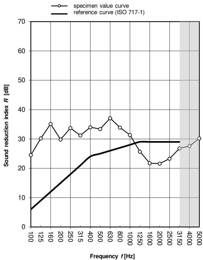
Graph 2 - Conf. 2
