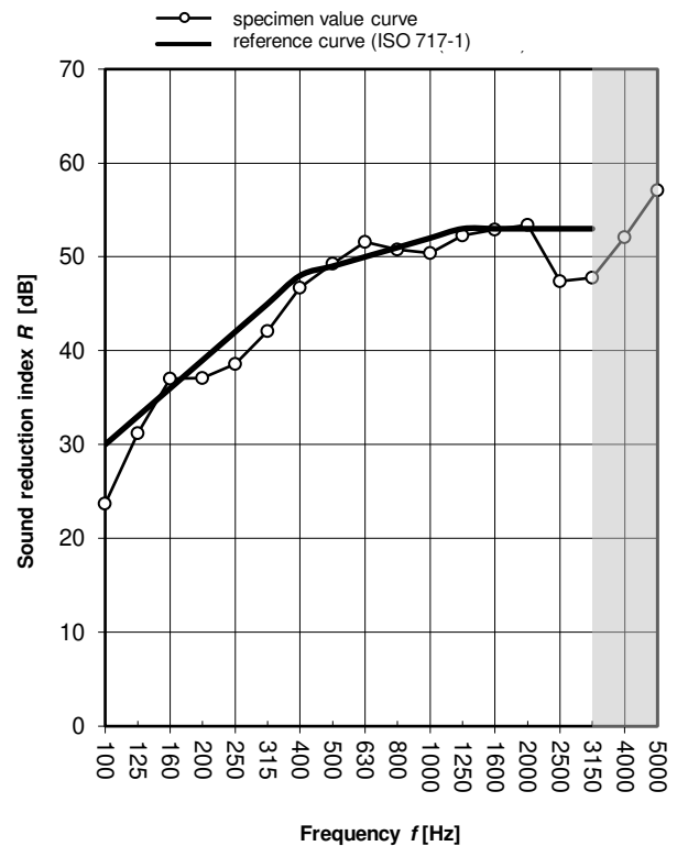
Graph 3 - Conf. 3
