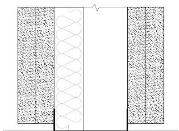
Figure 2 - Conf. 2 scheme
