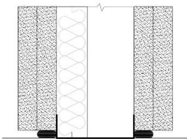
Figure 4 - Conf. 3 scheme
