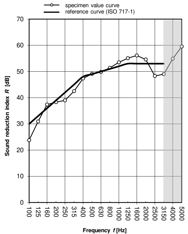
Graph 4 - Conf. 4
