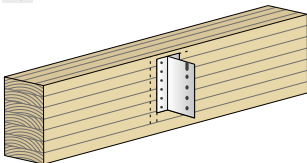
1b. Fix ALU bracket to main beam.
